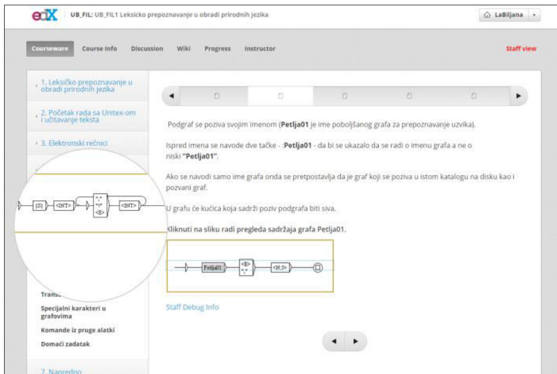
Image 1: Zooming subgraph
